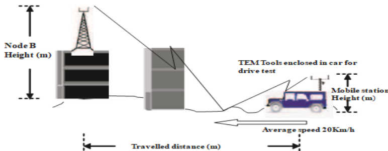
Fig. 1: Sketch of TEMS Drive Test Configuration
