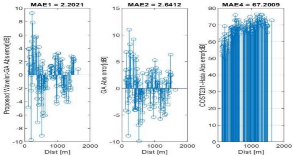
Figure 9: MAE of Wavelet-GA model, GA Model, and COST231-Hata in eNodeB Site 1
