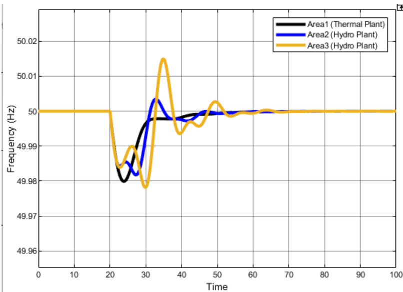
Figure 16 Load disturbance at both areas
