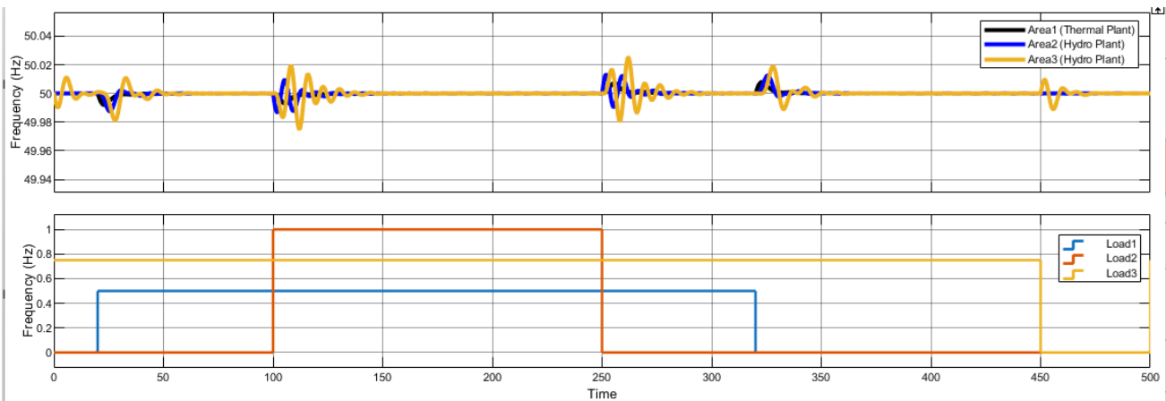
Figure 18 Frequency, Turbine speed and Load graph
