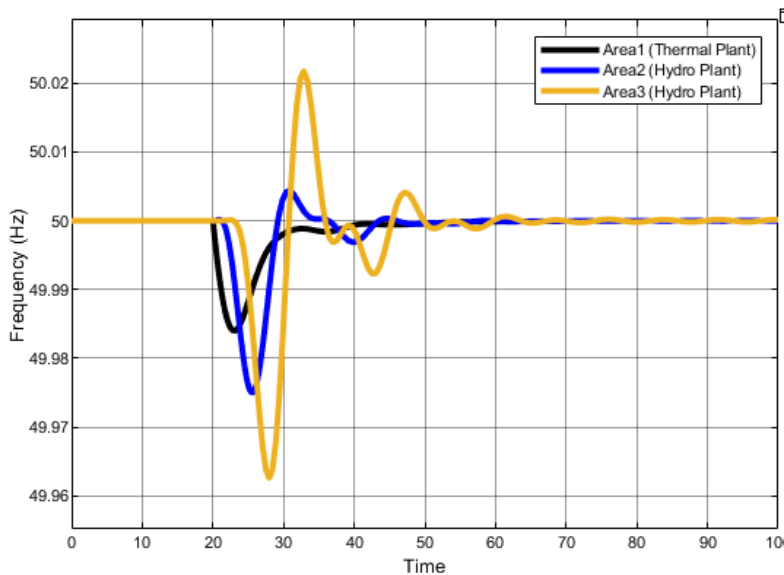
Figure 14 Load disturbance at area one only
