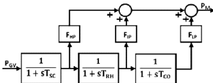
Figure 3 Steam turbine configuration (Nikhil et al., 2016) Figure 3 models a reheat tandem compound steam turbine where all three main components are captured in the model. These components are the SC, the RH and the CO.
