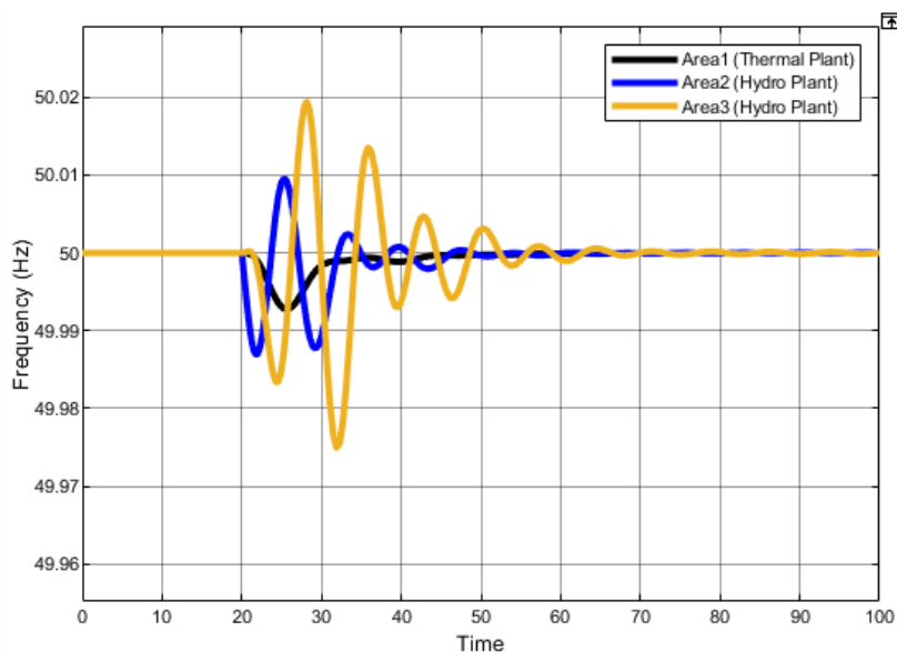
Figure 15 Load disturbance at area two only
