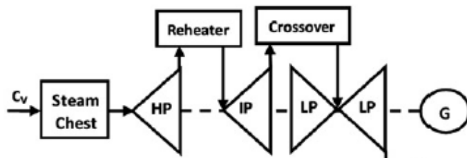
Figure 2 Steam turbine configuration (Nikhil et al., 2016)
