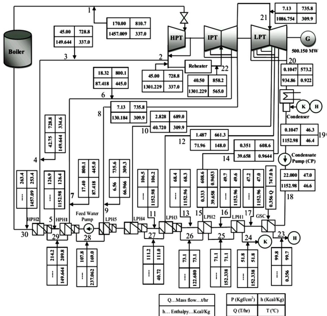
Figure 1 Heat balance diagram for a 500 MW thermal plant (Basu, 2018)
