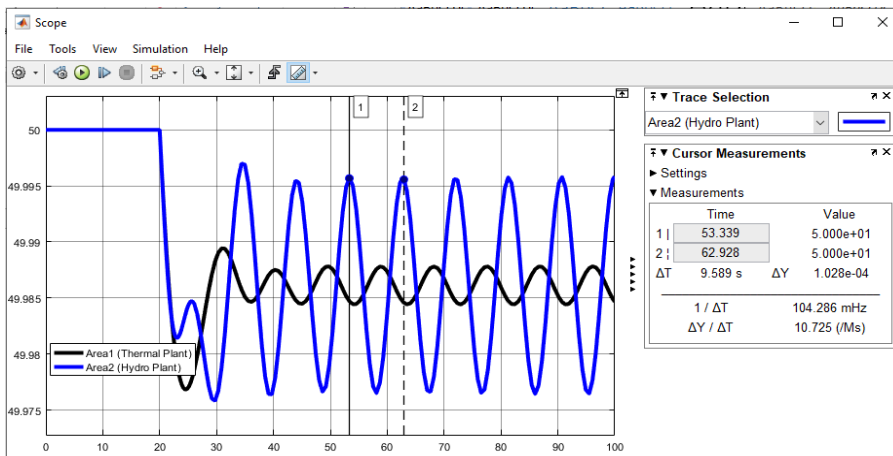
Figure 10 PID tuning area two
