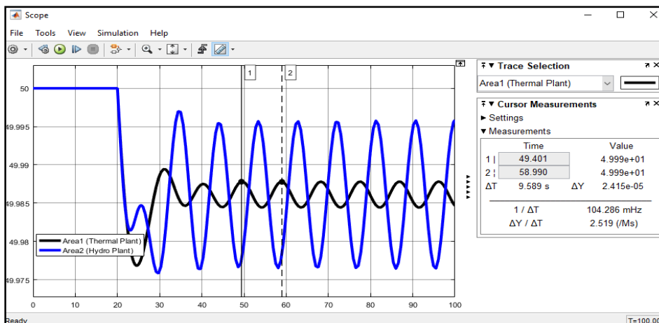
Figure 9 PID tuning area one
