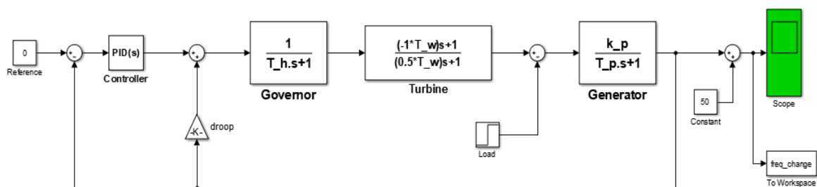
Figure 6 Hydro plant model
