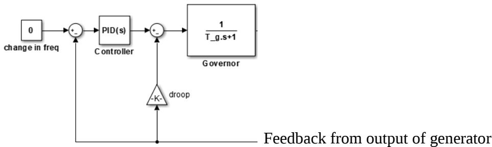
Figure 8 PID controller design
